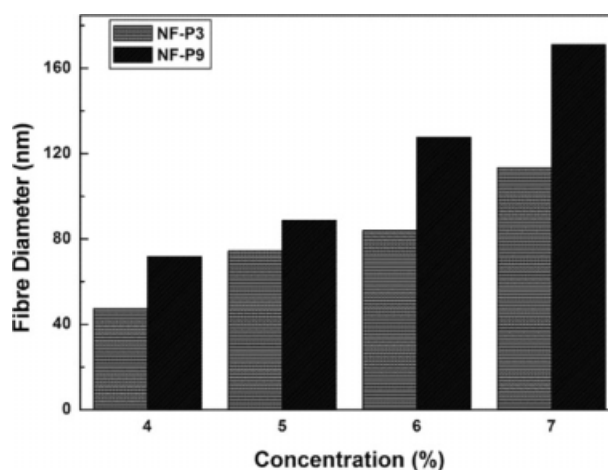
Figure 3 Comparison between concentrations (4–7%) and the corresponding average fiber diameter of electrospun nanofiber, PEO M_w = 3 \times 10^5 g/mol (NF-P3), 9 \times 10^5 g/mol (NF-P9) at 15 cm and applied voltage of 10 kV (0.6 kV/cm).
