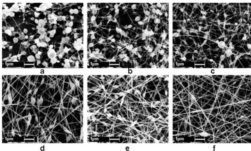
Figure 4 SEM images of electrospun nanofibers from (a) 5%, (b) 5%*, (c) 5%***, (d) 6%, (e) 6%*, (f) 6%** PEO ( M_w = 3 \times 10^5 g/mol) aqueous solution at 13 cm and applied voltage of 15 kV (1.15 kV/cm). * denotes with 2% PAA ** denotes with 2% PAH.
