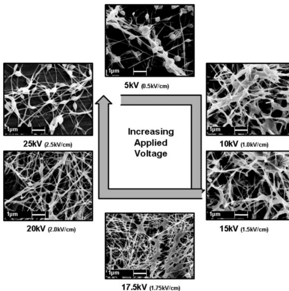
Figure 8 SEM micrographs showing the effect of an electric field on the microstructures of electrospun 7% PEO ( M_w = 3 \times 10^5 g/mol) solution at a tip-to-collector distance of 10 cm and at applied potential voltage of 5–25 kV (0.5 kV–2.5 kV/cm).
