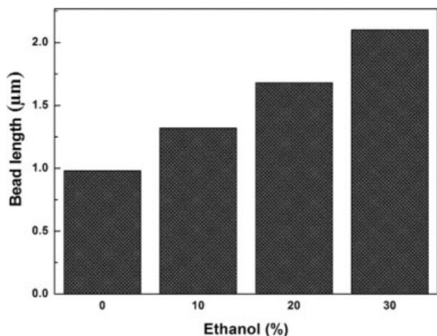
Figure 6 Relationship between the amount of Ethanol added to a 3% PEO ( M_w = 9 \times 10^5 g/mol) aqueous solution and the corresponding bead lengths of electrospun nanofibers at 20 cm and applied voltage of 5 kV (0.25 kV/cm).
