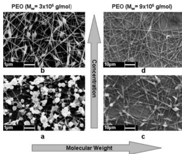
Figure 2 SEM micrographs showing the effect of molecular weight on the microstructures of electrospun nanofibers from (a) 5%, (b) 6% PEO ( 3 \times 10^5 g/mol) aqueous solution; (c) 5%, (d) 6% PEO ( M_w = 9 \times 10^5 g/mol) aqueous solution at 15 cm and applied voltage of 10 kV (0.6 kV/cm). All other parameters were kept constant.
