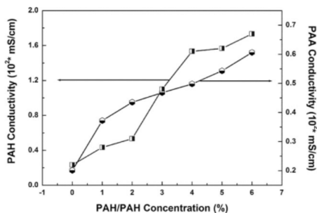
Figure 5 The effect of polyelectrolyte on the conductivity of 6% PEO ( M_w = 3 \times 10^5 g/mol) aqueous solution at 13 cm and applied voltage of 15 kV (1.15 kV/cm).
