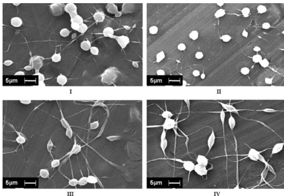
Figure 7 SEM micrographs showing the effect of ethanol added to a 3% PEO ( M_w = 9 \times 10^5 g/mol) aqueous solution on the morphology of electrospun nanofibers (I) 0%; (II) 10%; (III) 20%; (IV) 30% ethanol at 20 cm and applied voltage of 5 kV (0.25 kV/cm).
